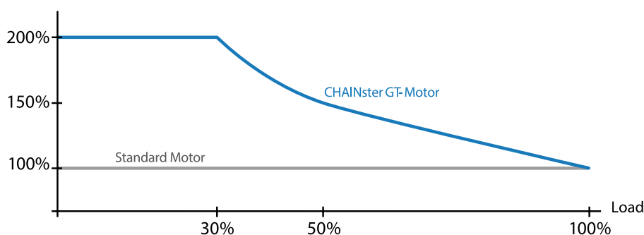
Hoisting Speed
