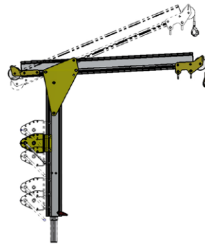
Standard Type W (Winch and Shackle) T-DAVIT
