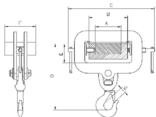
Modelo TZH, swivel hooks, pivoting and swivelling
