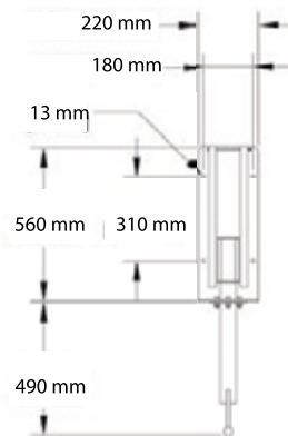
Shown with Optional Adjustable Height Wall Bracket
